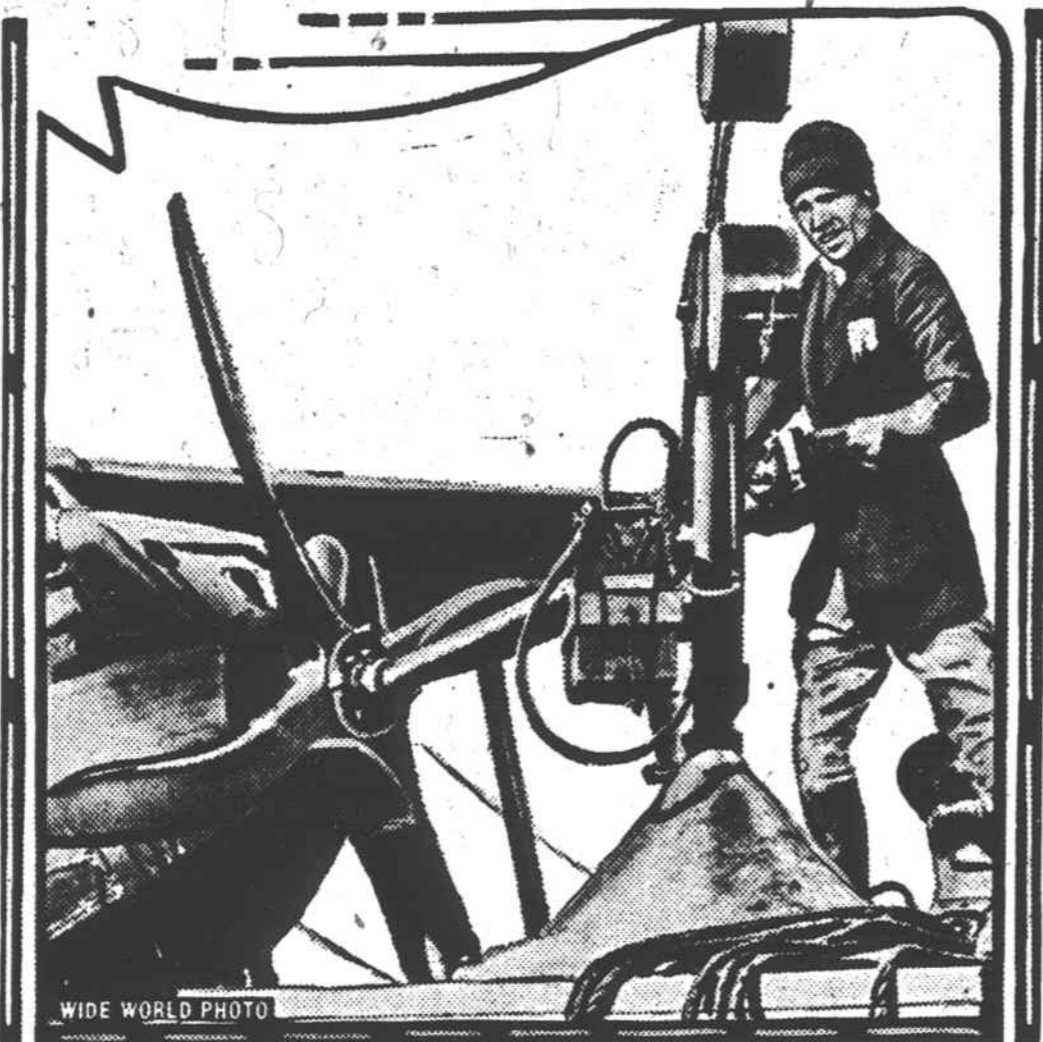
A new device for the starting of a plane has just been introduced at McCook field in Dayton, O., which practically eliminates the danger of the old method of turning the propeller by hand. The device is fastened to a motor truck and is brought on the field and fastened to the propeller which is spun with the turning on of the "juice."
