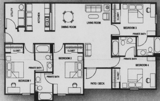
4 Bedroom Floorplan
