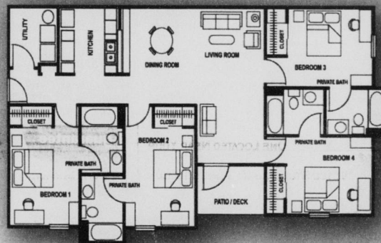
4 Bedroom Floorplan
