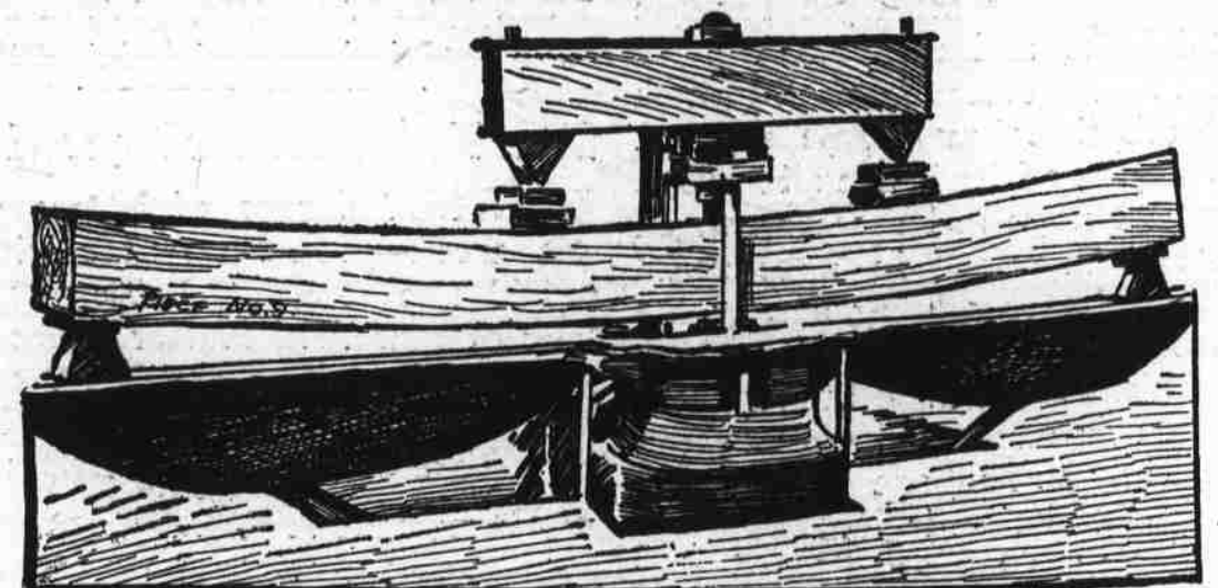
A Government Machine for Testing the Strength of Wood
