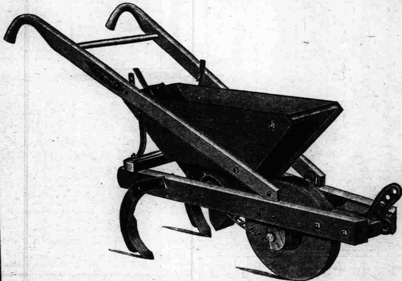
THE COLE DOUBLE FOOT GUANO DISTRIBUTOR AND LISTER.
