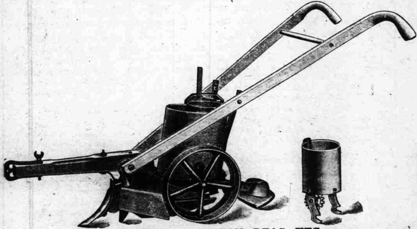
No. 5.—FOR CORN, COTTON, PEAS, ETC.
