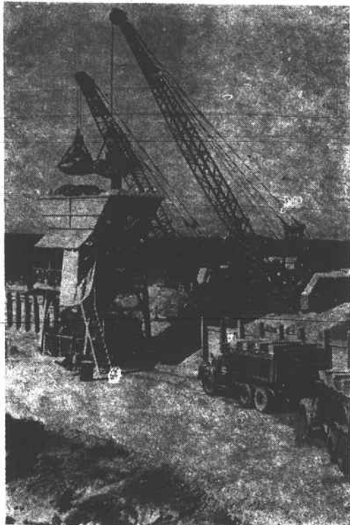
Above paving machine is seen in operation near Oine. To the left mixer is mixing aggregate as power scoops pour stone and sand into hopper. Nearby, but not shown, is concrete mixer loading a stream of trucks. (Staff Photos)
