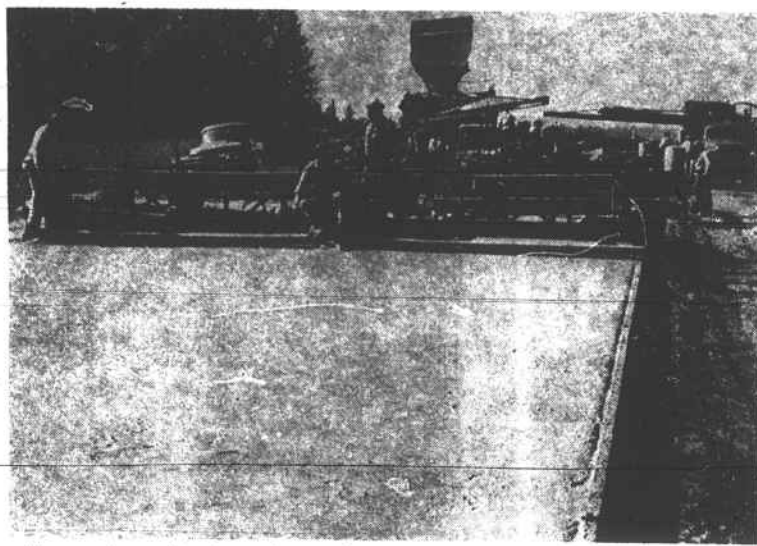
Above paving machine is seen in operation near Oine. To the left mixer is mixing aggregate as power scoops pour stone and sand into hopper. Nearby, but not shown, is concrete mixer loading a stream of trucks. (Staff Photos)
