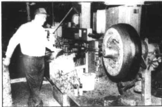
An orbitread machine allows our personnel to use bulk rubber in preparing all of the hot caps. This modern machine applies 16 pounds of rubber a minute to the tires, and allows for recapping a tire with no splice, making for a better balanced, smoother tire.
