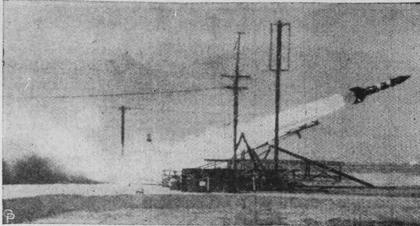
LEAVING ITS RAMP AT THE NAVAL ORDNANCE test station, Inyokern, Calif., is a new type of booster rocket. It is believed to be the world's largest solid propellant rocket yet flown. It will be employed in launching supersonic missiles, relying on the new ram-jet engine of the Navy for a propulsion unit. Note the gap between the rocket and burning gases behind it.
