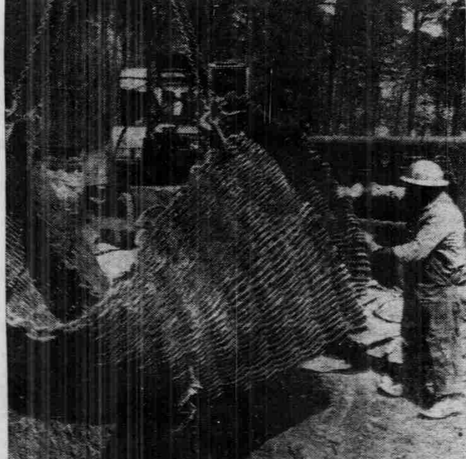
... and a "dynamite mat" is lowered into the foundation to prevent the explosion from throwing rocks out of the area. Then, the wires are connected to the detonator and the blast is set off... leaving rubble.
