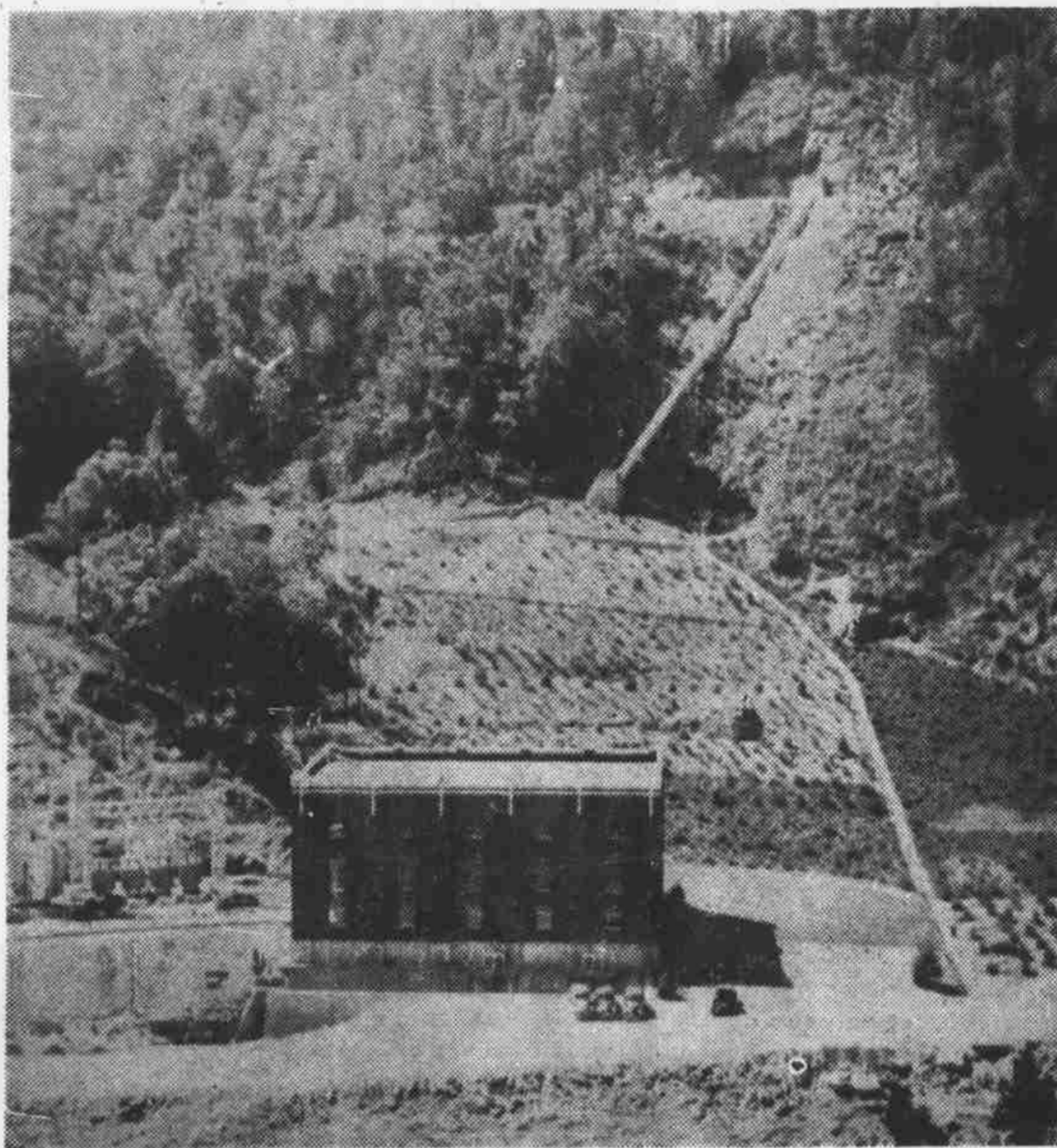
This red brick, steel and concrete structure of modern architectural design, set in solid rock, is 56 by 112 feet in plan and 101 feet high from foundation to parapet. It houses the generating unit and its valves. The control room is two stories underground. This hydro-electric power unit of the Nantahala Power and Light company is located on the west fork of the Tuckasee river in Jackson County.
