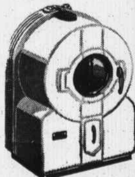
STANDARD MODEL
