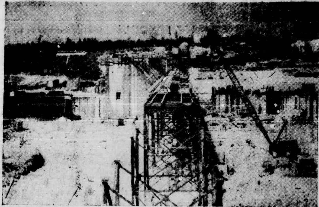
Buggs Island Dam construction has commenced in the second stage cofferdam. The above photograph shows the construction trestle being built in the second stage cofferdam area; this construction trestle is used to transport the construction material to the site of activity. In the background may be seen the partially complete concrete piers constructed in the first stage cofferdam with the huge concrete mixing plant, aggregate refrigeration plant and aggregate storage piles. To the left background may be seen the observation platform from which construction activities may be observed by visitors to the project.
