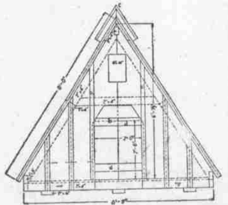
Front of A-Shaped House.
