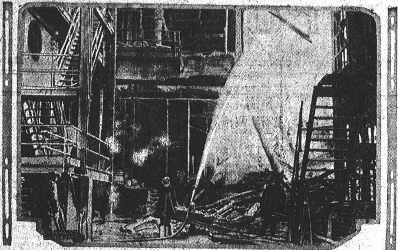
Scene in the ruins of the starch plant of the Corn Products company in Pekin, Ill., after the terrific dust ex- plosion which killed 36 employees and injured many others.
