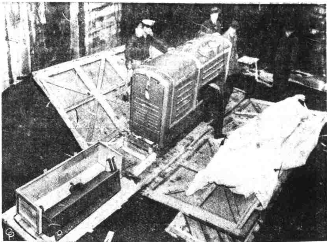
IF THE DUQUESNE LIGHT COMPANY WORKERS go on strike and cause a shutdown of power in Pittsburgh, the Shadyside Hospital is ready to meet the emergency. Here a sixty-horsepower Diesel generator, purchased from Army surplus, is uncrated for installation at the hospital. The union, representing 3,400 workers, seeks a wage increase of 29 cents an hour. The company has offered 7 1/2 cents. (International Soundphoto)
