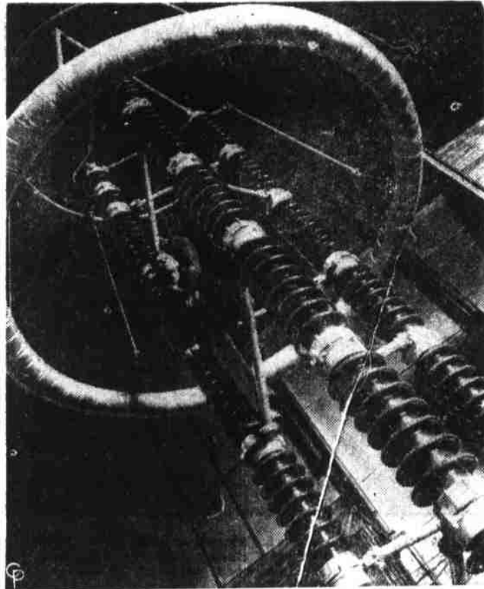
LARGEST lightning arrester ever built, this forty-foot experimental model can handle any bolt from the old Scandinavian god Thor's thunderbolts. Nearing completion at Trafford, Pa., it will be installed in the new 500,000 volt test transmission line being built by the American Gas and Electric Company near Steubenville, Ohio, to provide information on the best type of protection for such lines. (International)
