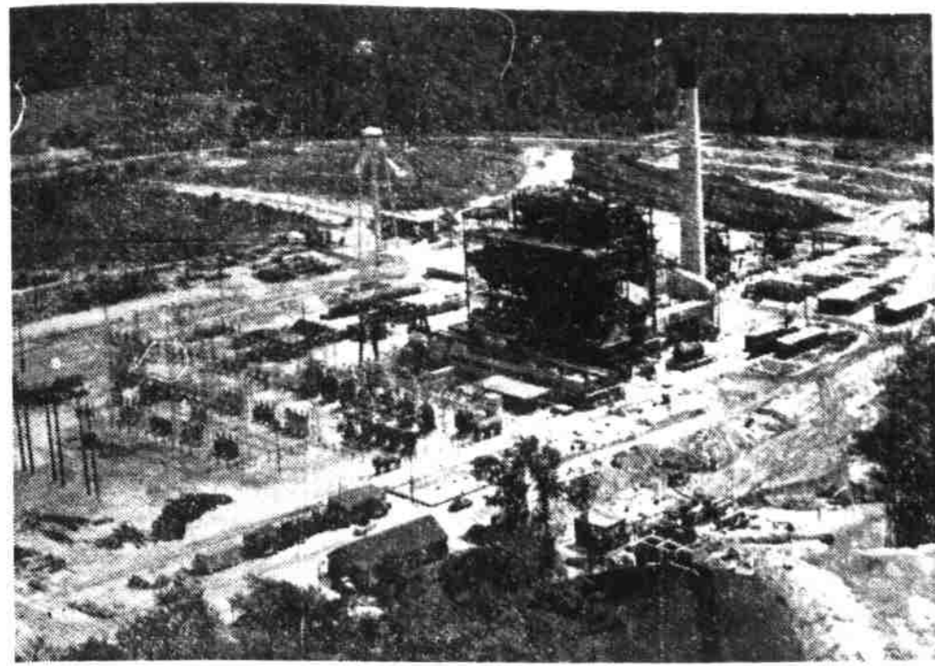
Latest instrument for development of the Carolinas is this 120,000-horse-power steam electric generating plant at Lenoir, which will be put in service by the Carolina Power & Light Co. September 30th. The first 100,000-kw. unit of the plant, which is a similar unit and a similar unit is being installed. The Lenoir plant is part of a $200,000,000 expansion program underway by CP&L. It will provide over 740,000,000 kilowatt-hours of electricity per year, enough to serve over 300,000 average residences.
