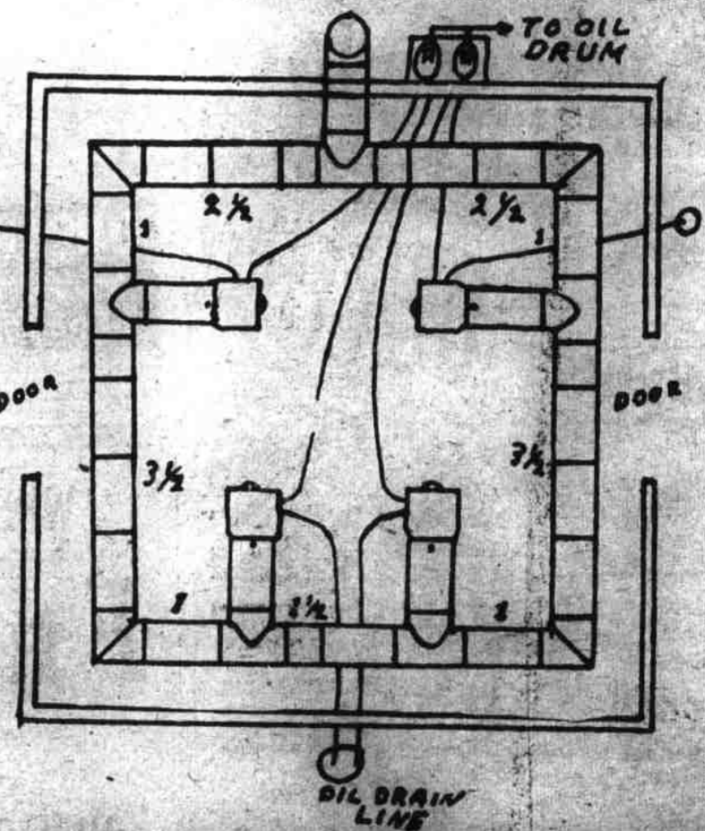
FLUE & BURNER ARRANGEMENT FOR 16' BARN
