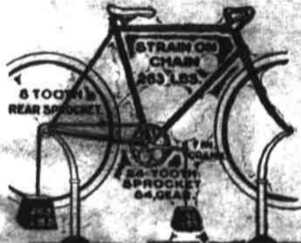
Note the enormous increase in the strain smaller sprockets and a 4-inch lower gear.
