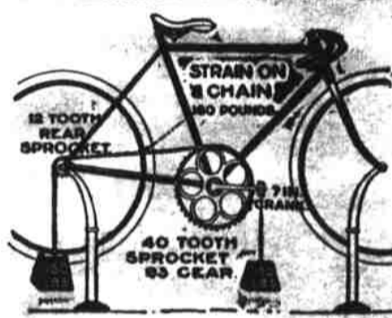
The Fastest Hill Climber in the World. Only 10 lbs more strain on chain than on pedals.
