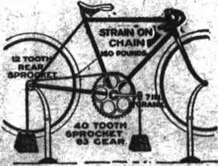
The Easiest Hill Climber in the World. Only 10 lbs more strain on chain than on pedals. A STANDARD HIGH-GRADE BICYCLE.
