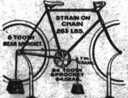
Note the enormous increase in the strain smaller sprockets and a 9-inch lower gear.
