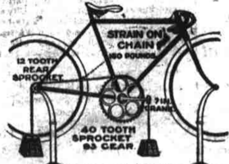
The Easiest Hill Climber in the World. Only 10 lbs more strain on chain than on pedals. A STANDARD HIGH-GRADE BICYCLE.
