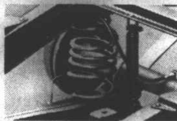
TOUGH COIL SPRINGS FRONT AND REAR ON 1-1/2- AND 1-1/4-TON MODELS
