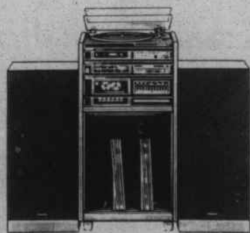
Panasonic SC-3000 FM/AM Stereo Receiver with Built-in Cassette Recorder, Semi-Automatic Turntable, Tower Speakers, and Rack. All-in-one rack system with quartz synthesizer FM/AM digital tuner and 6 FM/6 AM station preset buttons. Also includes 5-segment LED level meters for both the left and right channels and a front-loading cassette deck system. Belt-drive auto-return turntable with DC motor. Standard-type rack with casters.
