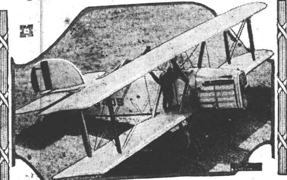
This is one of the airplanes of the Douglas DT-2 type especially built for the proposed round-the-world flight of United States army air service aviators.
