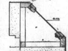
Hotbed for basement window well. Cross sections show how it fits window. (Masonite Design)
