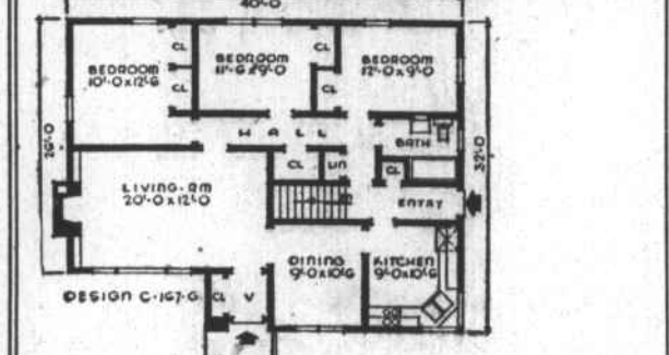
A SMALL HOUSE PLANNING BUREAU DESIGN NO. C-167-G.
