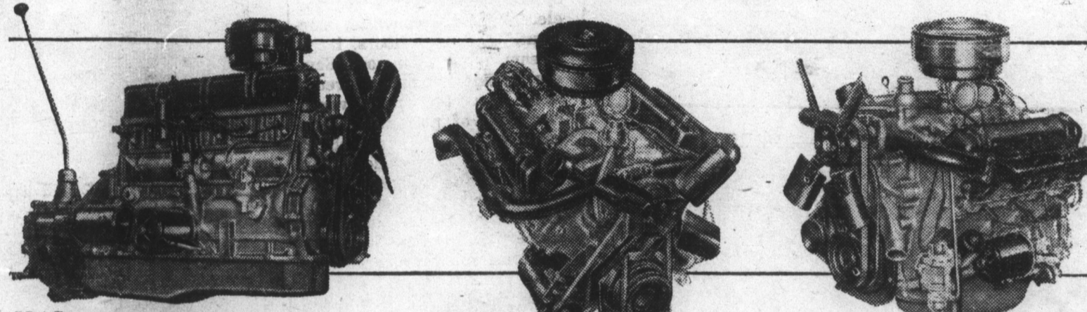
F.D.A.F. 101-H.P. COST CLIPPER SIX; New LOW-FRICTION design. 212 cu. in. Available Series F-1 thru F-5. 145-H.P. CARGO KING V-8; New LOW-FRICTION design. 279 cu. in. Standard in Series F-7. 155-H.P. CARGO KING V-8; New LOW-FRICTION design. 317 cu. in. Standard in Series F-8.
