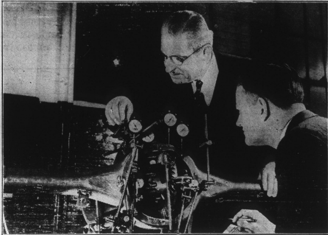
Means of this unique test on a passenger car rear axle, set up in the laboratory of the Chevrolet Gear and Axle Plant in Detroit, twelve gauges measure every possible deflection assumed by the parts in the rear axle under a given load condition. A weight is hung on the end of the drive shaft that corresponds to a maximum load on the axle during actual driving conditions. All movements or deflections of the drive shaft, pinion and ring gears, and axle shafts are then read simultaneously. Such minute and constant checking results in better mounting of bearings, that serves to prolong axle life and insure more satisfactory service. In this picture are Leo B. Olick (left) and Jack Kelly.
