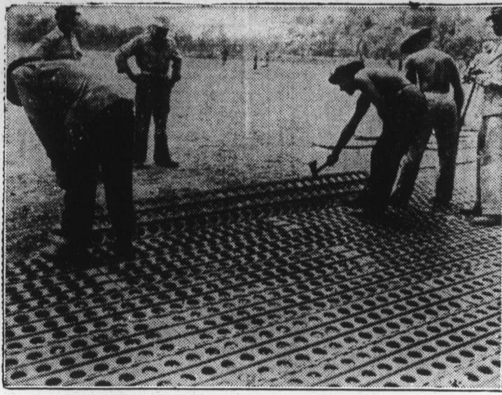
Bureau of Public Relations U. S. War Department NEW GUINEA —Landing fields for bombers, pursuit and fighter planes are quickly constructed by the Engineers utilizing the interlocking steel mat. This construction is elastic in handling and thoroughly durable for the use intended.
