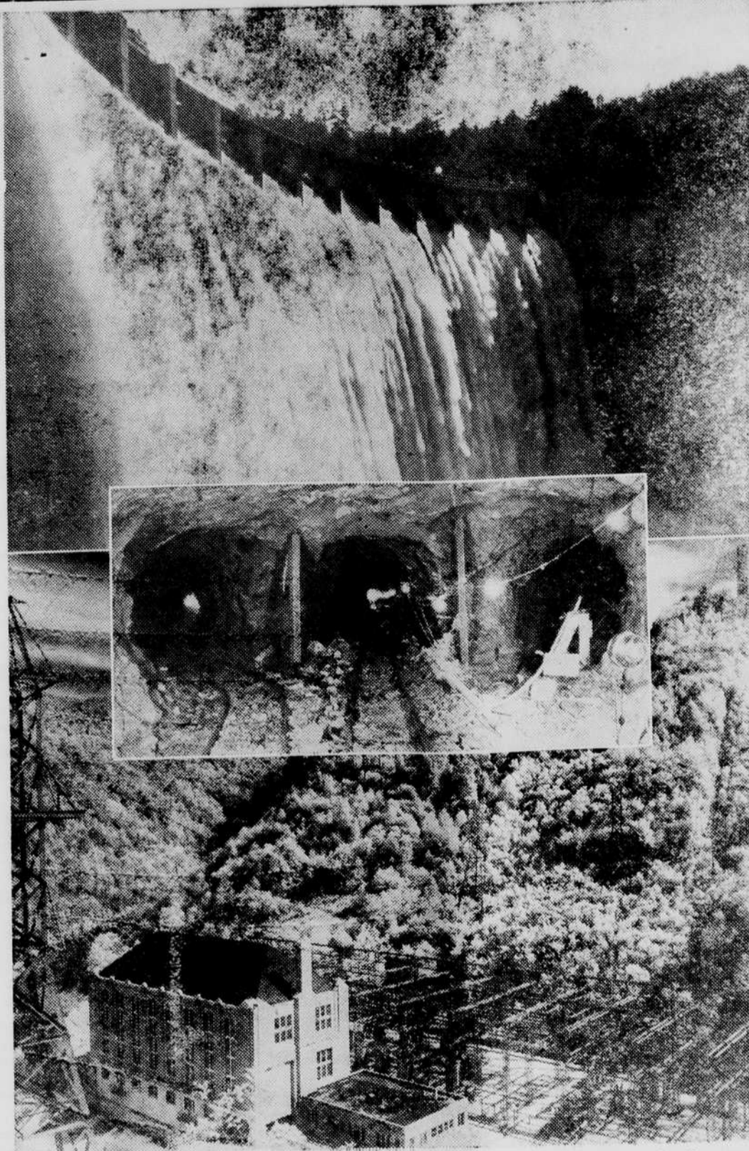
PIONEERING POWER PROJECT —Carolina Power & Light Company gained national recognition with its Waterville hydroelectric development on the Pigeon River. The dam (top) had the highest head of water east of the Mississippi, and a tunnel (inset) was punched through six miles of mountain to deliver water to the generating plant (below). The Waterville unit, later named for Vice-President C. S. Walters, went into operation in 1930. It has a capacity of 145,000 horsepower.
