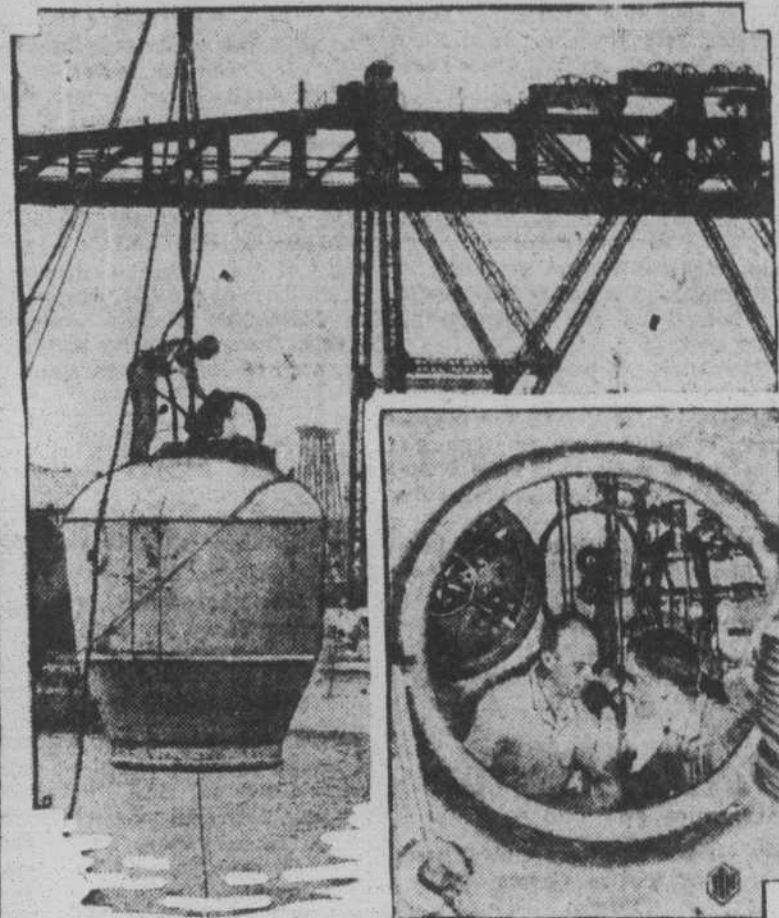
Under the watchful eyes of United States Naval officers, the newly invented and perfected submarine diving bell or rescue chamber is shown above being lowered into the water at Brooklyn, N. Y., Navy Yard for a test. As many as eight men at a time can be transferred from a sunken vessel to the chamber, which rises to the surface from its own buoyancy. Lieut. Commander A. P. McCann and Lieut. A. M. Morgan (insert) show how telephone communication can be carried on with ships on the surface from the interior of the bell.
