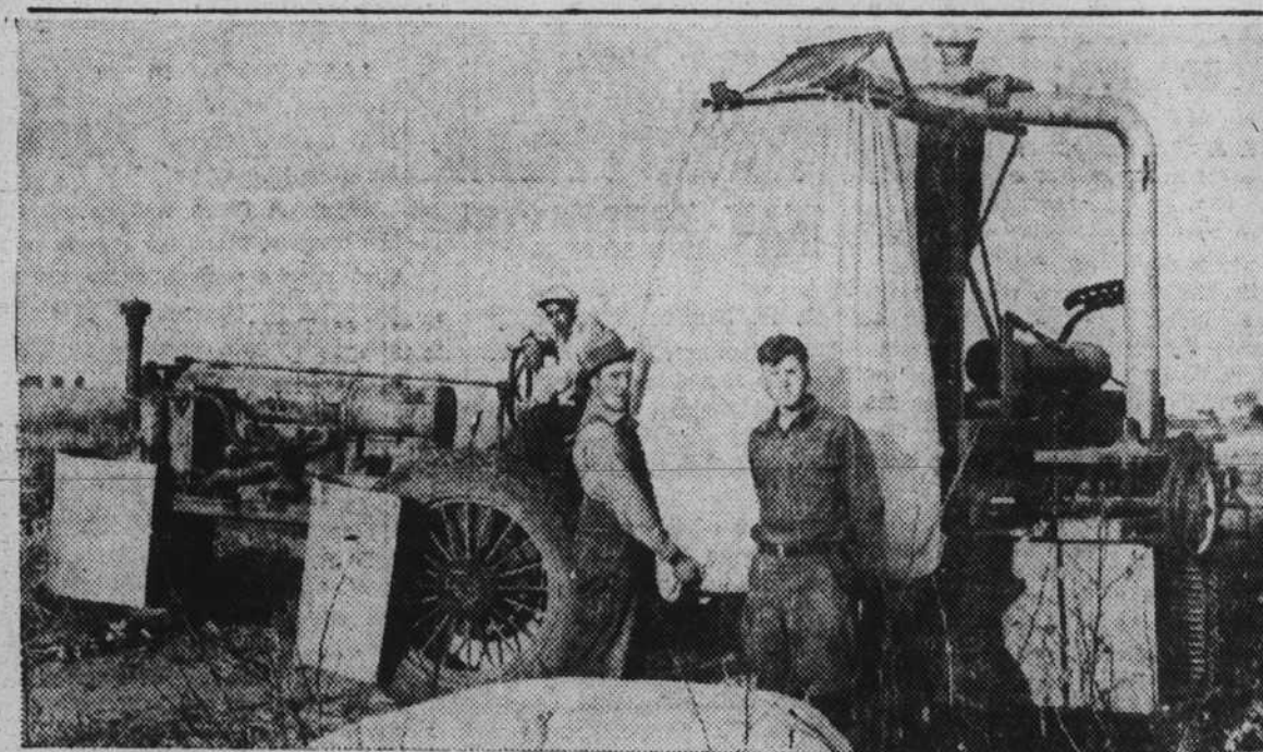
TO REVOLUTIONIZE COTTON INDUSTRY? —This cotton picking machine, being tested on irrigated fields in the Salt River valley of Arizona, may revolutionize the industry. Built by J. D. and M. D. Rust, of Memphis, Tenn., it has an ingenious system of claw-like spindles to rip the cotton from the pods. Another apparatus removes the cotton from these spindles and a blower attachment carries the cotton to the waiting sack. The machine picks 1,400 pounds of cotton an hour. M. D. Rust is shown in the foreground (hatless).
