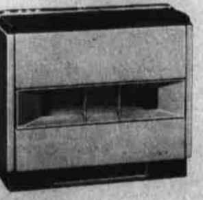
DELUXE UNIT. Features *CAST IRON COMBUSTION CHAMBER and BURNER; floor level heat from INTERNAL BLOWER, with motorized outlets; no "ceiling draft"; *TOP RETURN *PUSH BUTTON control (for motorized louvers).
