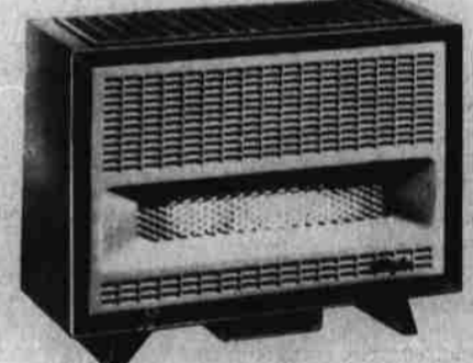
CUSTOM GAS HOME HEATING UNIT. Has CAST IRON slotted burners (in STEEL COMBUSTION CHAMBER) *EXHAUST PORTS *FINGER TIP DIAL SETTING *TWO SPEED BLOWER *FLOOR HEAT OUTLET.
