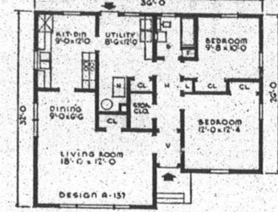
THE AUSTEN , a basementsless house, features easy circulation. All rooms can be reached from either front or rear entrance without passing through any room. A dining alcove, with large double windows, is a part of the living room which has
