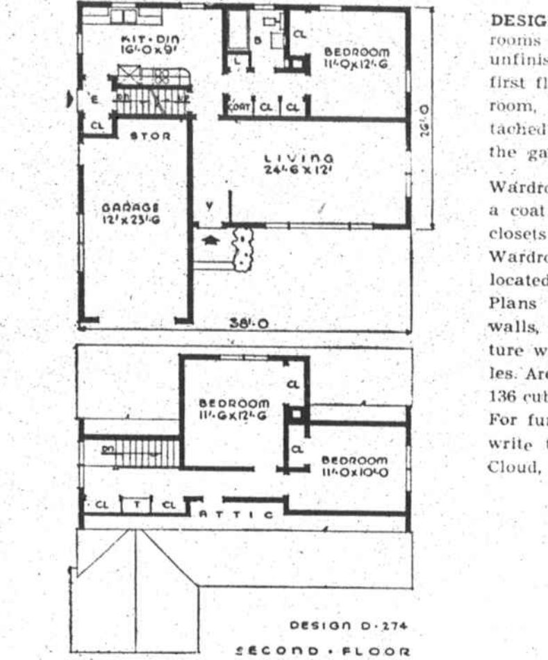
A SMALL HOUSE PLANNING BUREAU DESIGN NO. D-274
