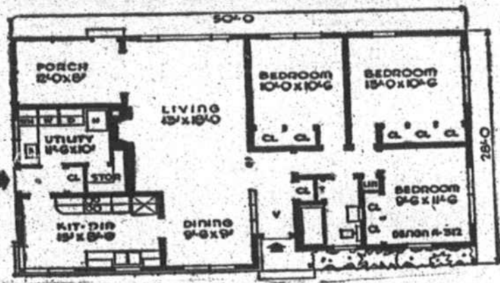
A SMALL HOUSE PLANNING BUREAU DESIGN NO. A-312
