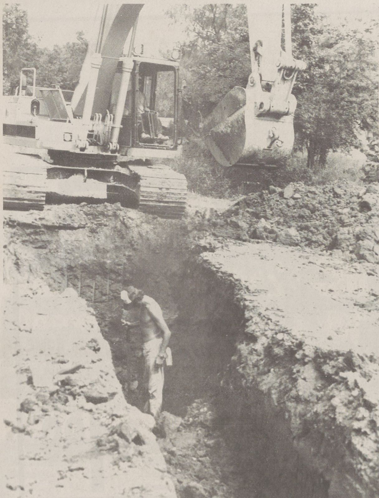
BRIDGES DRIVE PROJECT -City workers begin preliminary work for sewer construction on Bridges Drive, Phase I of the major construction project, which also includes running of water lines and drainage improvements. Robert Putnam, on back hoe, Emmett Rhodes, in the ditch, and William Young, right, begin work on the project which will take months to complete.
