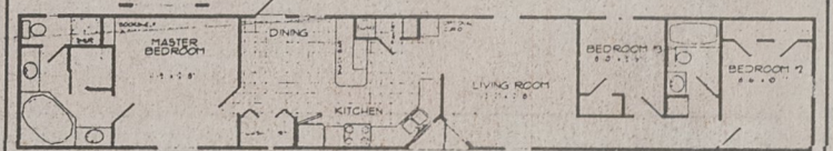
Sample Floor Plan 14' X 80'
